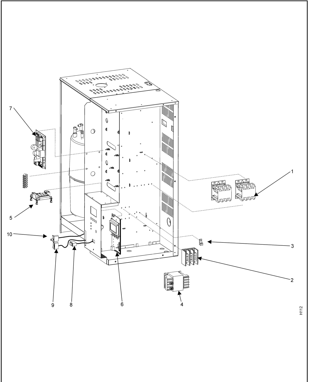
Figure 8. NHTC/NHPC Electrical Compartment Exploded View and Spare Parts
